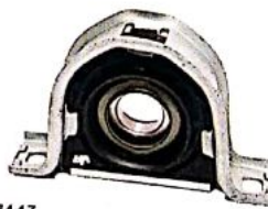
2215 7443 248 CJR BEARING 6207 ASSEMBLY WITH BRACKET
